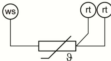
Figure 1: Electrical connection
