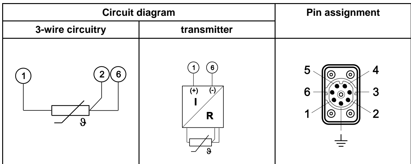
Figure 1: Variants of electrical connection
