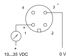
Connection diagram transmitter
