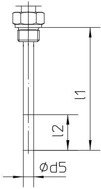
shanks, fixed G1/2B, G3/4B, 1/2" NPT D1107/1109/1122
