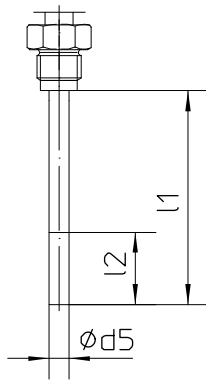
shanks rotating, G1/2B D1207
