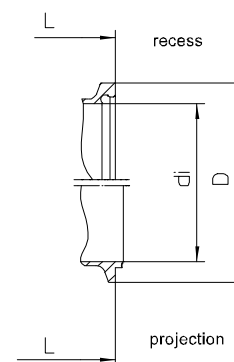
clamp connection
