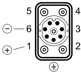
2-wire technology
