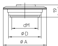
VARIVENT ® connection for VARINLINE ® case
